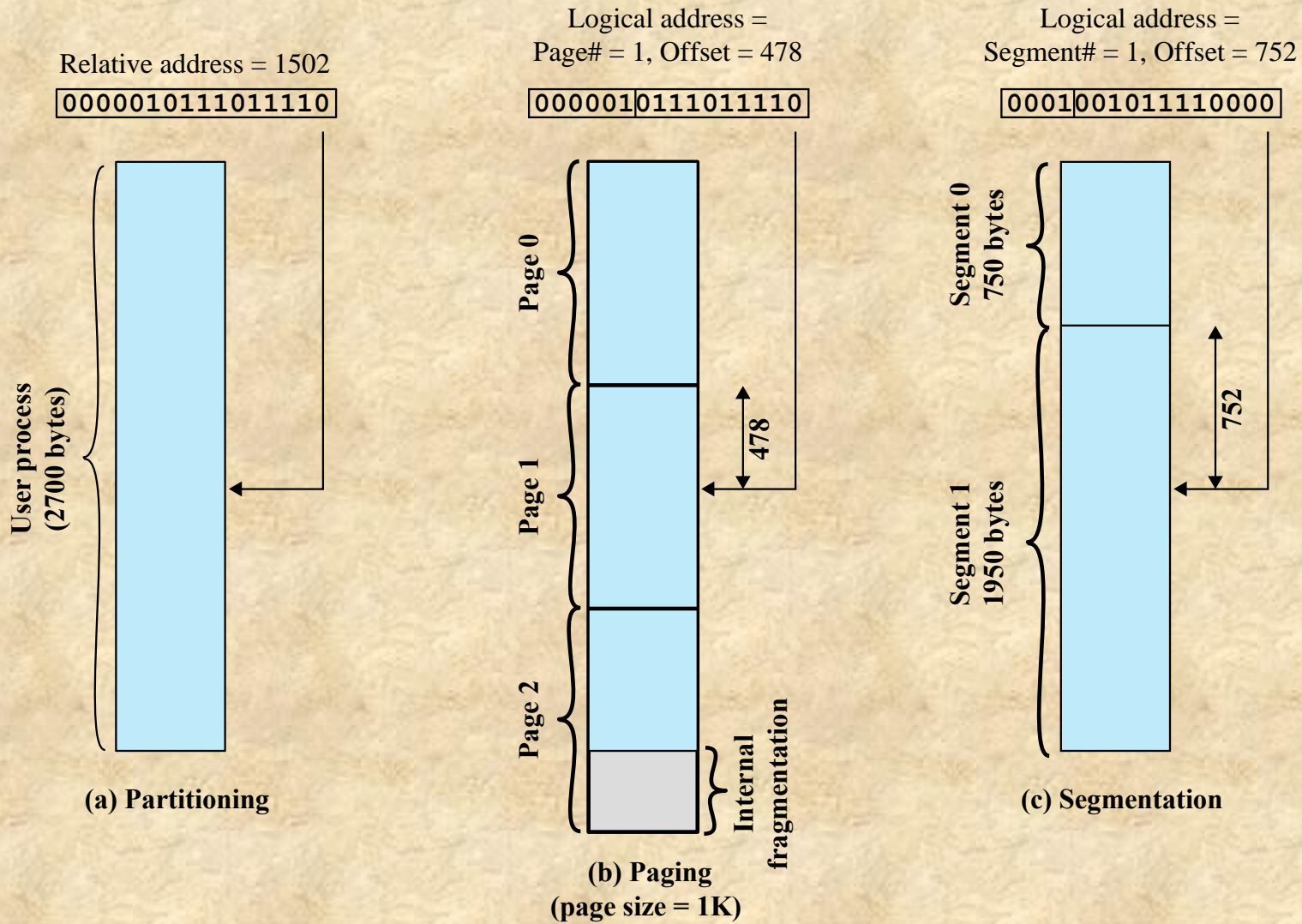
Figure 7.11 Logical Addresses
